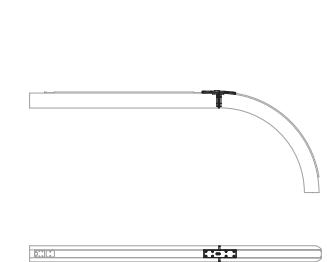
15. Code 2265010A LINEAR - 90° VERTICAL DOWN JOINT
