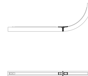
14. Code 2264010A LINEAR - 90° VERTICAL UP JOINT
